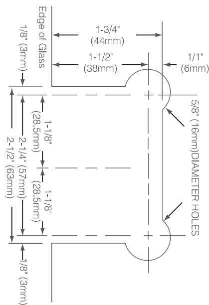
180° GLASS TO GLASS
