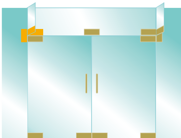
TYPICAL STORE ENTRANCE WITH SUPPORT FINS (Viewed from the Inside)
