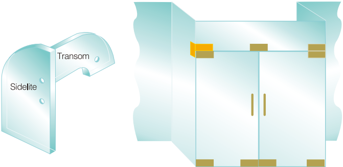
TYPICAL RECESSED STORE ENTRANCE (Viewed from the Inside)
