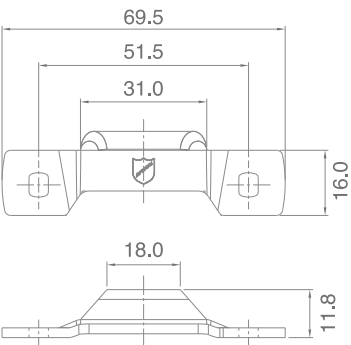
Casement hinge protector low
