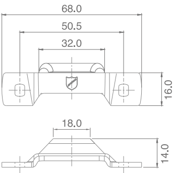
Casement hinge protector high
