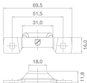
Casement hinge protector low
