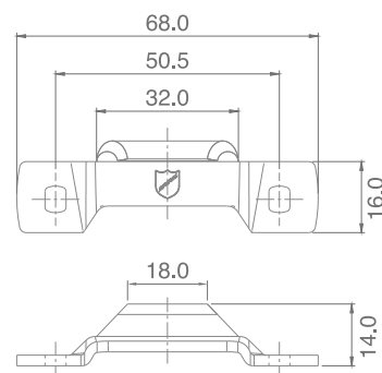
Casement hinge protector high
