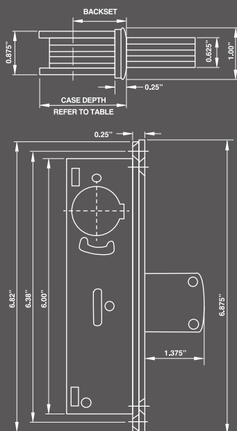
DEADBOLT
